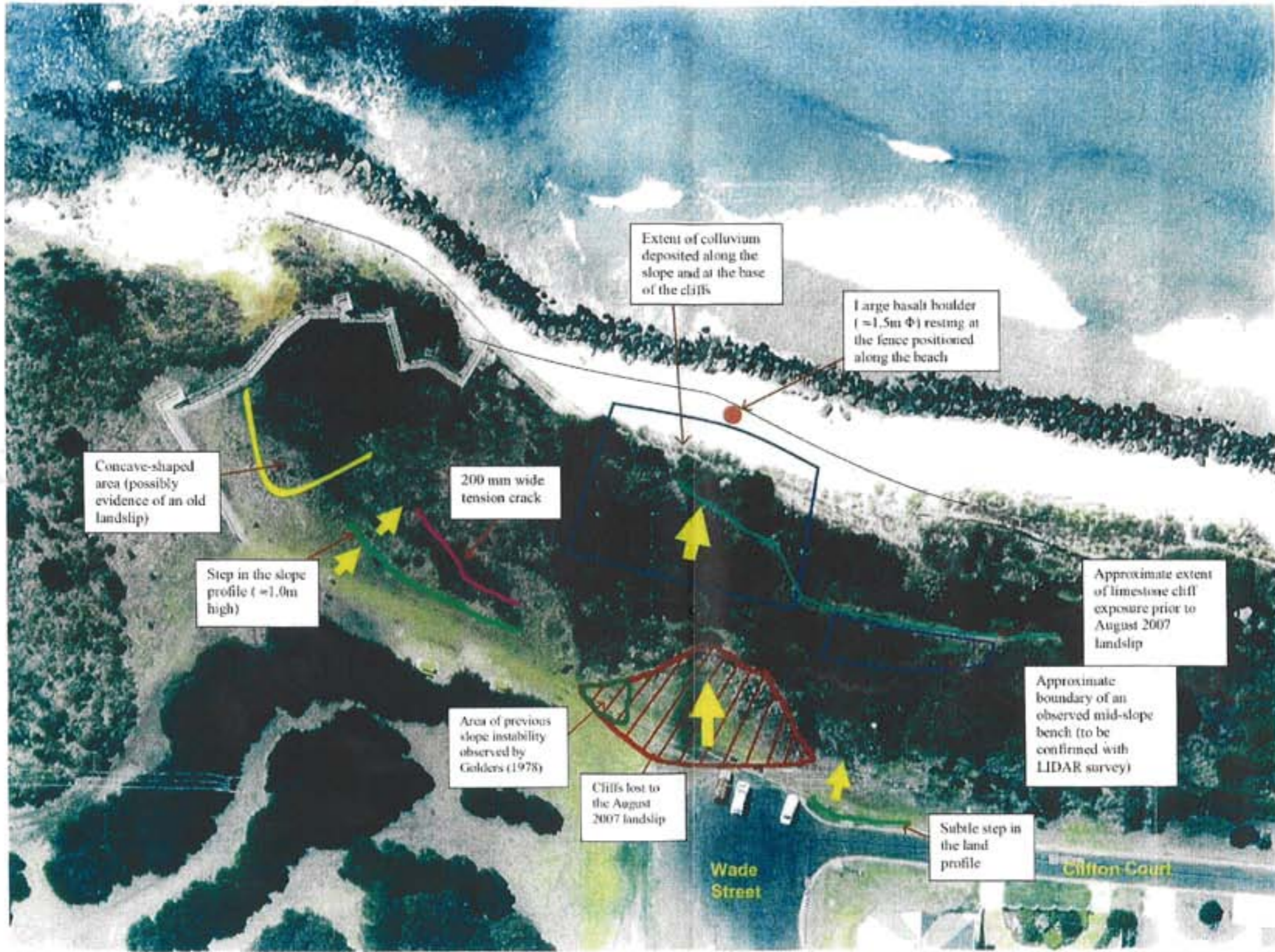
Portland Wade Street Slip Department of Sustainability and Environment Aerial Photograph of Key Land Slip Features December 2008
